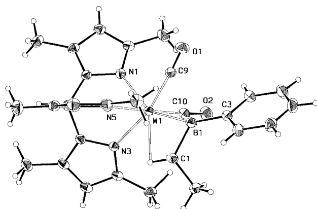
Fig. 7 Molecular structure of complex 16b . Selected bond lengths [ \text{\AA} ] and angles [ ^\circ ]: W1–B1 2.070(4), W1...C1 2.476(4), W1–C9 1.941, W1–C10 1.951(4), W1–N1 2.183(3), W1–N3 2.255(3), W1–N5 2.257, B1–C1 1.619(5), B1–C3 1.557(5), C9–O1 1.168(4) and C10–O2 1.174(4); W1–B1–C1 83.4(2), W1–B1–C3 154.7(3), W1–C9–O1 176.3(3), W1–C10–O2 177.2(3) and C1–B1–C3 121.7(3).
