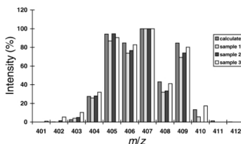
Fig. 2 Experimental and calculated ( n = 0 , 86%, n = 1 , 14%; M^+ 84%, [ M - H ] + 16%) mass distributions of the parent ion of [W( \eta -C 5 Me 5 )(CO) 2 (C 2 H 2 + n D 3 – n )] 11b-D , generated from complex 2-D with 1.7 equivalents of “HBET 2 ”. Experimental data from three separate mass spectroscopic analyses are shown.
