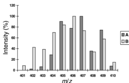
Fig. 3 Experimental mass distributions of the parent ions of [\text{W}(\eta\text{-C}_5\text{Me}_5)(\text{CO})_2(\text{C}_2\text{H}_2 + n\text{D}_3 - n)] 11b-D , generated from complex 2-D with 1.7 (A) and 3.4 equivalents of “ \text{HBEt}_2 ” (B), respectively.
