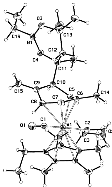
Fig. 4 Molecular structure of complex 14 . Selected bond lengths [Å] and angles [°]: W1–C1 1.959(5), W1–C2 2.222(5), W1–C5 2.330(6), W1–C6 2.260(6), W1–C7 2.244(5), W1–C8 2.365(5), C1–O1 1.160(5), C2–O2 1.218(5), C2–C3 1.543(6), C5–C6 1.436(6), C6–C7 1.417(6), C6–C14 1.509(6), C7–C8 1.424(6), C8–C9 1.479(6), C9–C10 1.525(6), C9–C15 1.337(6), C10–C11 1.560(6), C11–C12 1.525(6), C11–O4 1.457(5), C12–C13 1.531(6), C13–O3 1.458(6), B1–O3 1.359(6), B1–O4 1.363(6) and B1–C19 1.579(7); W1–C1–O1 174.9(4), W1–C2–O2 123.4(3), W1–C2–C3 119.6(3), O2–C2–C3 117.0(4), O3–B1–O4 123.7(4), O3–B1–C19 119.3(4) and O4–B1–C19 117.0(4).
